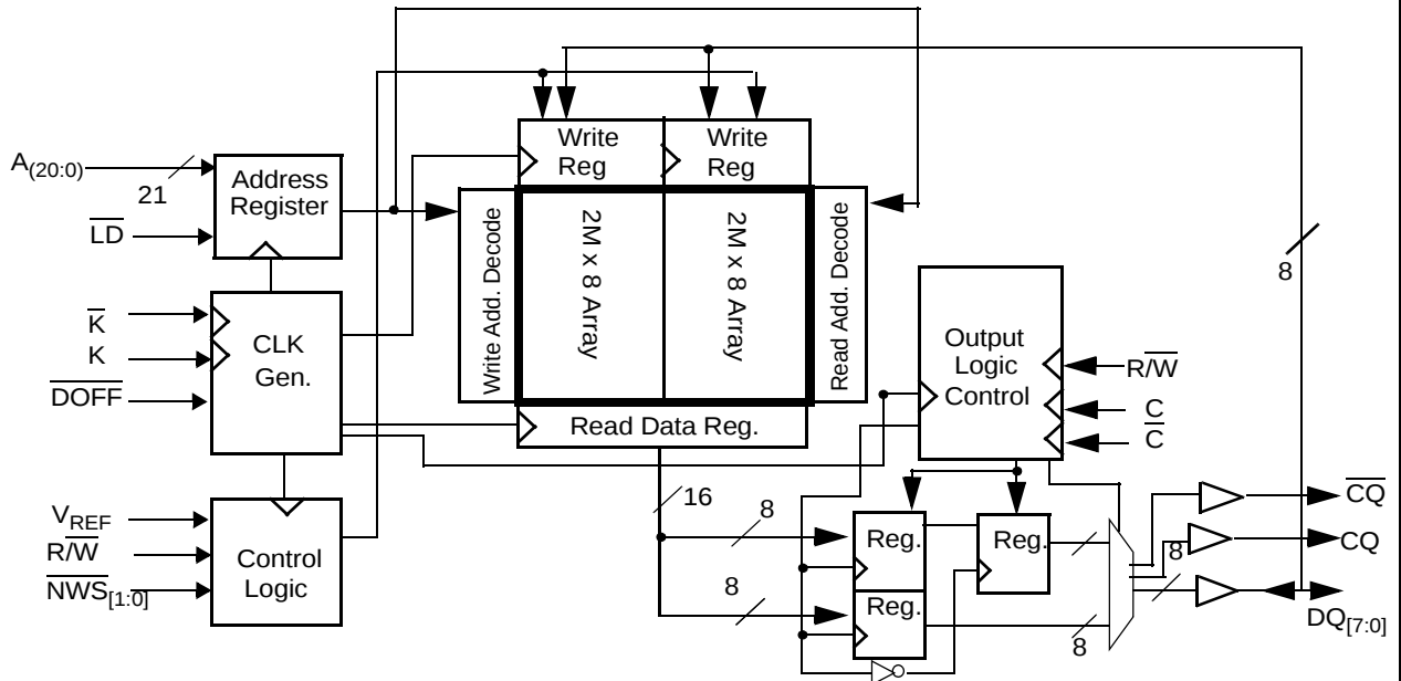
Logic Block Diagram (CY7C1416AV18)
