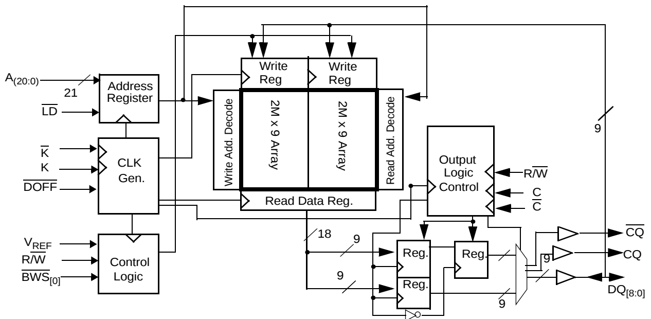
Logic Block Diagram (CY7C1427AV18)
