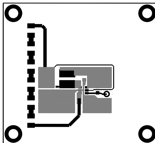
Figure 4: Top Layer
