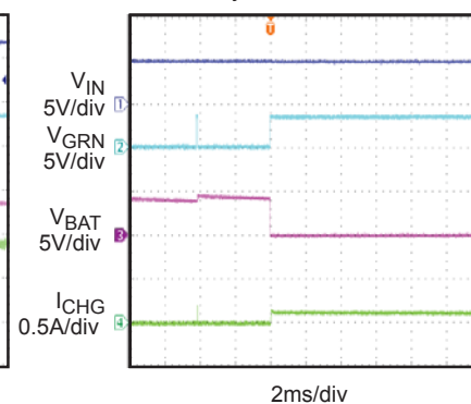
Short Circuit
