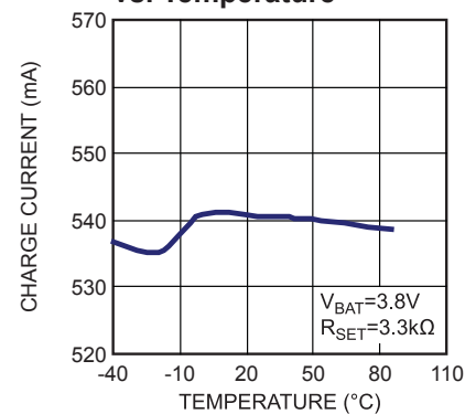
Constant Current Charge vs. Temperature
