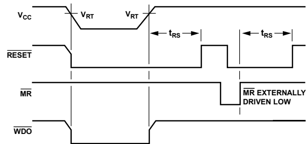
Figure 15. \text{RESET} , \overline{\text{MR}} , and \text{WDO} Timing
