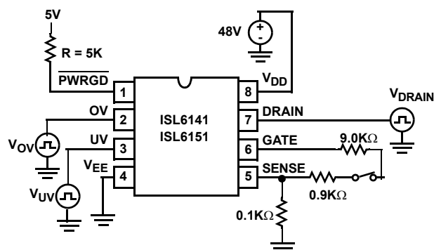
FIGURE 2B. TEST CIRCUIT FOR 600μs TIME-OUT
