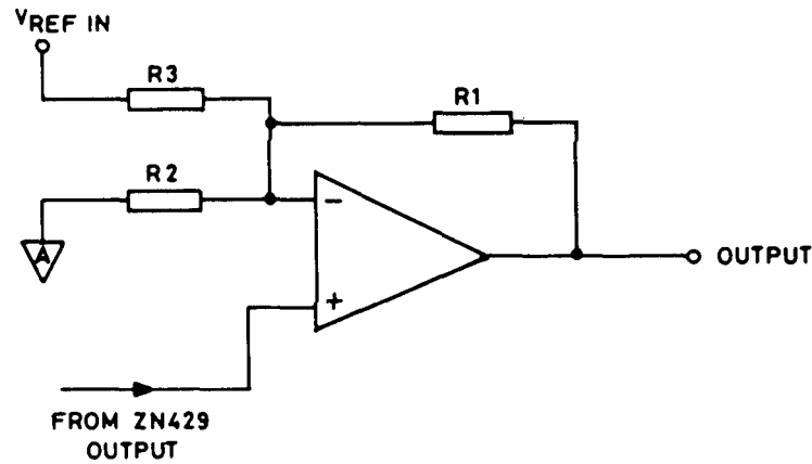
Fig.6 Bipolar operation - basic circuit
