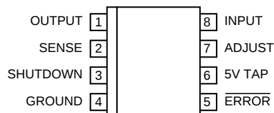
MIC29204BM (SO-8)
