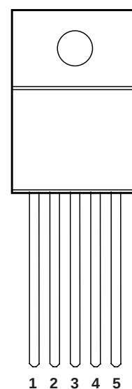
MIC29201/29202BT (TO-220-5)
