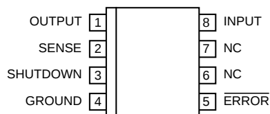
MIC29201-3.3BM (SO-8)
