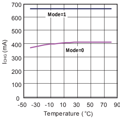
CC Charge Current vs. Temperature
