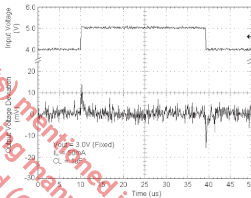
Fig. 37: Line Transient Response
