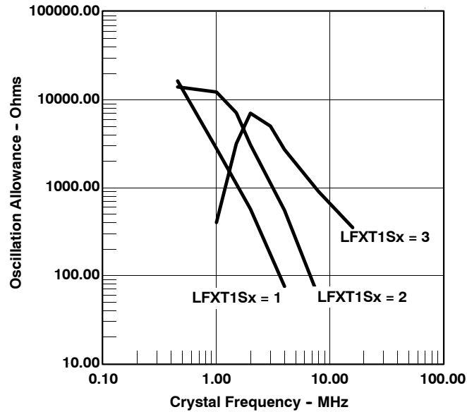
Figure 23. Oscillation Allowance vs Crystal Frequency, C_{L,eff} = 15 \text{ pF} , T_A = 25^\circ\text{C}
