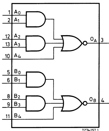
Fig.1 Functional diagram.
