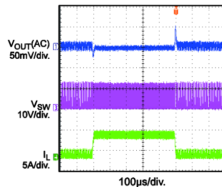
Transient I_{OUT}=0.6A-5.4A@2.5A/\mu s , F_{SW}=530kHz , C_{OUT}=3x22\mu F
