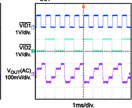
VID On-the-fly I_{OUT}=6A F_{VID1}=1kHz , F_{VID2}=0.5kHz , V_{OUT}=1.05V/1.1V/1.15V/1.2V
