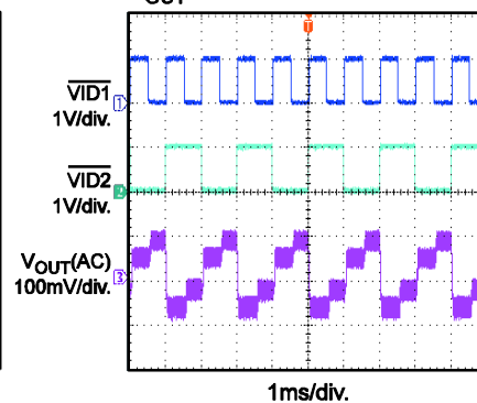
VID On-the-fly I_{OUT}=0.3A F_{VID1}=1kHz , F_{VID2}=0.5kHz , V_{OUT}=1.05V/1.1V/1.15V/1.2V
