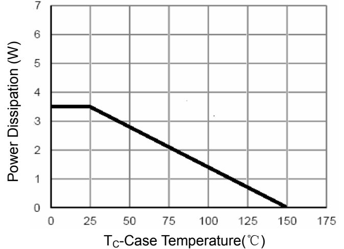
Figure 9 Power De-rating
