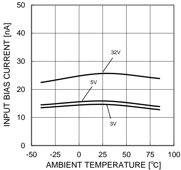
Figure 16. Input Bias Current - Ambient Temperature ( V_{ICM}=0V , OUT=1.4V )
